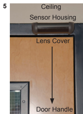
Install R2E-100 with Lens Cover Facing Down Toward Door Handle
