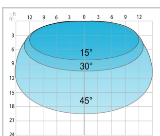
FALCON EXWIDE Mounting height: 11.5 ft
