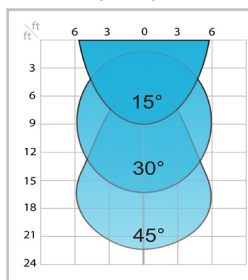
FALCON EX Mounting height: 16 ft
