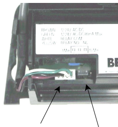
4-Wire Connector Auto-Learn Time Jumper
